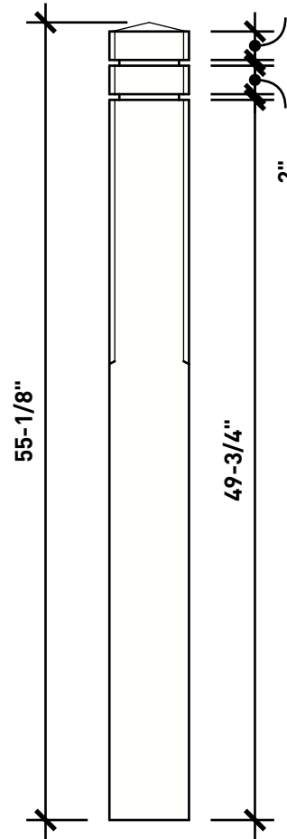
BOLLARD WITH 2 REVILES
